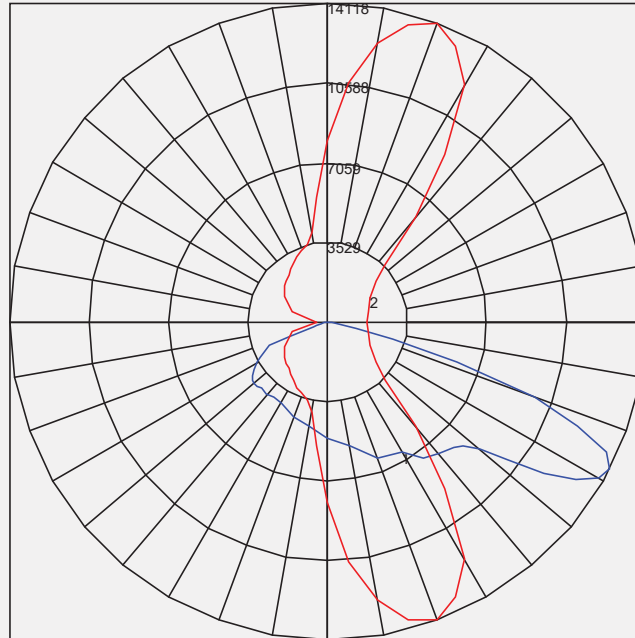
EYETINERA 250 NAV-T.IES POLAR GRAPH
