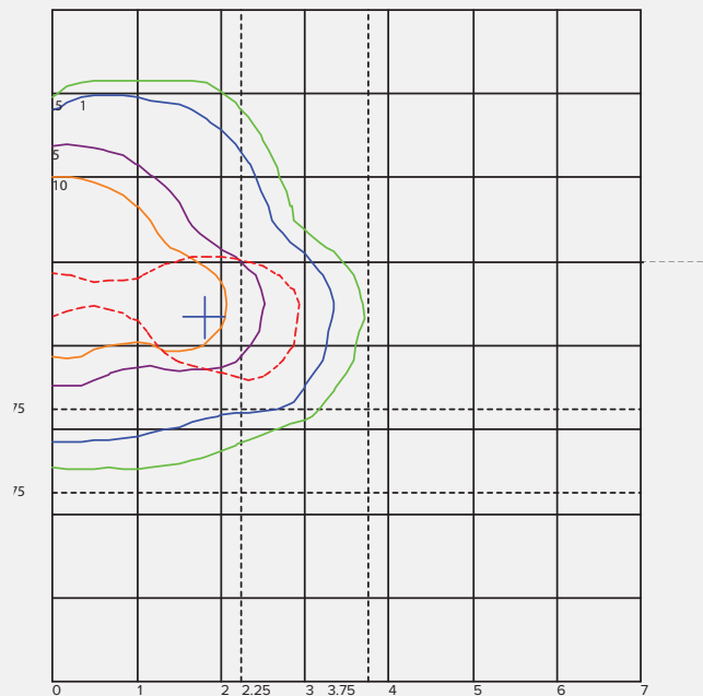
EYETINERA 250 NAV-T.IES ISOLUX LINES OF HORIZONTAL ILLUMINANCE
