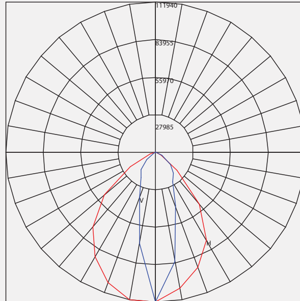
HP15 1000 HPS-T WB.IES AXIAL CANDELA DISPLAY
