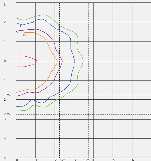
HP15 1000 HPS-T WB.IES SOLUX LINES OF HORIZONTAL ILLUMINANCE
