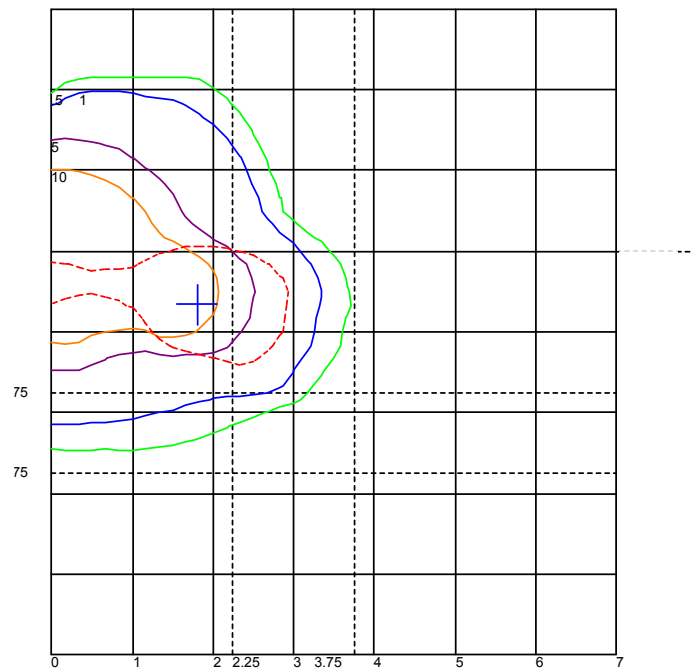
EYETINERA 250 NAV-T.IES ISOLUX LINES OF HORIZONTAL ILLUMINANCE
