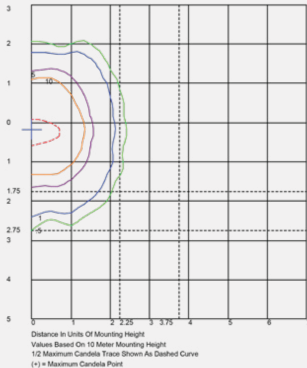
HP10 400 HPS WB.IES SOLUX LINES OF HORIZONTAL ILLUMINANCE
