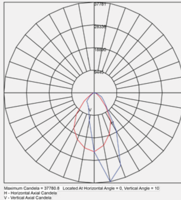
HP10 400 HPS WB.IES AXIAL CANDELA DISPLAY
